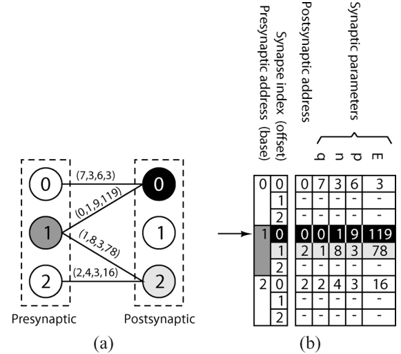
Fig. 1. (a) Virtual synapses: address-domain connectivity between presynaptic and postsynaptic neurons. Numbers in parentheses correspond to the synaptic parameters ( q , n , p , and E ) defined in Section II. (b) Lookup table storing addresses and parameters of the synaptic connections in random-access memory. The address of a presynaptic action potential “event” is used as an index into the table to identify postsynaptic target addresses and their corresponding synaptic parameters [1].
